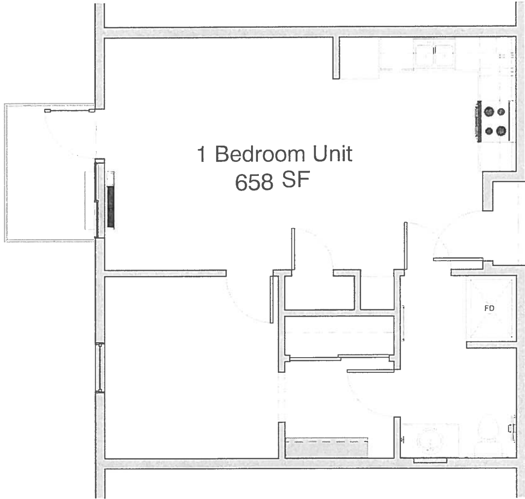
① Enlarged Plan - 1 Bedroom Unit - 3/16 3/16" = 1'-0"
